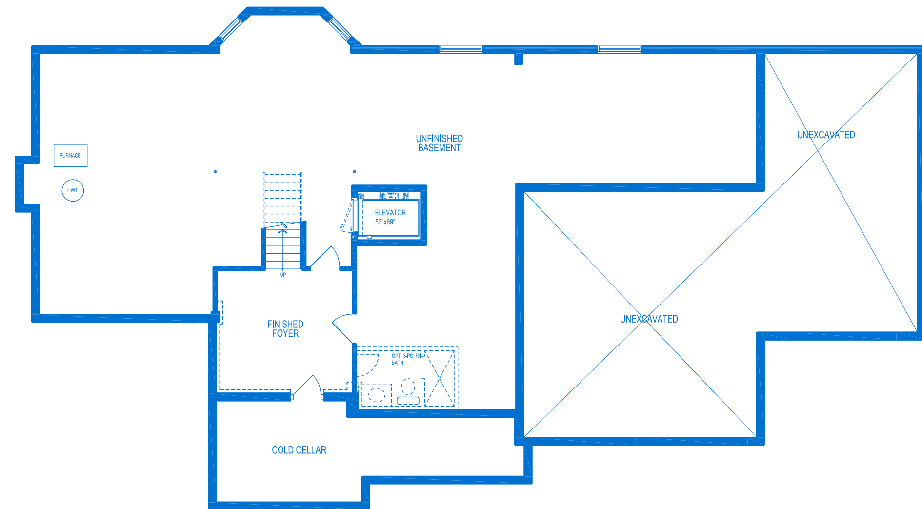
BASEMENT PLAN, ELEV. 'C' W/ ELEVATOR
