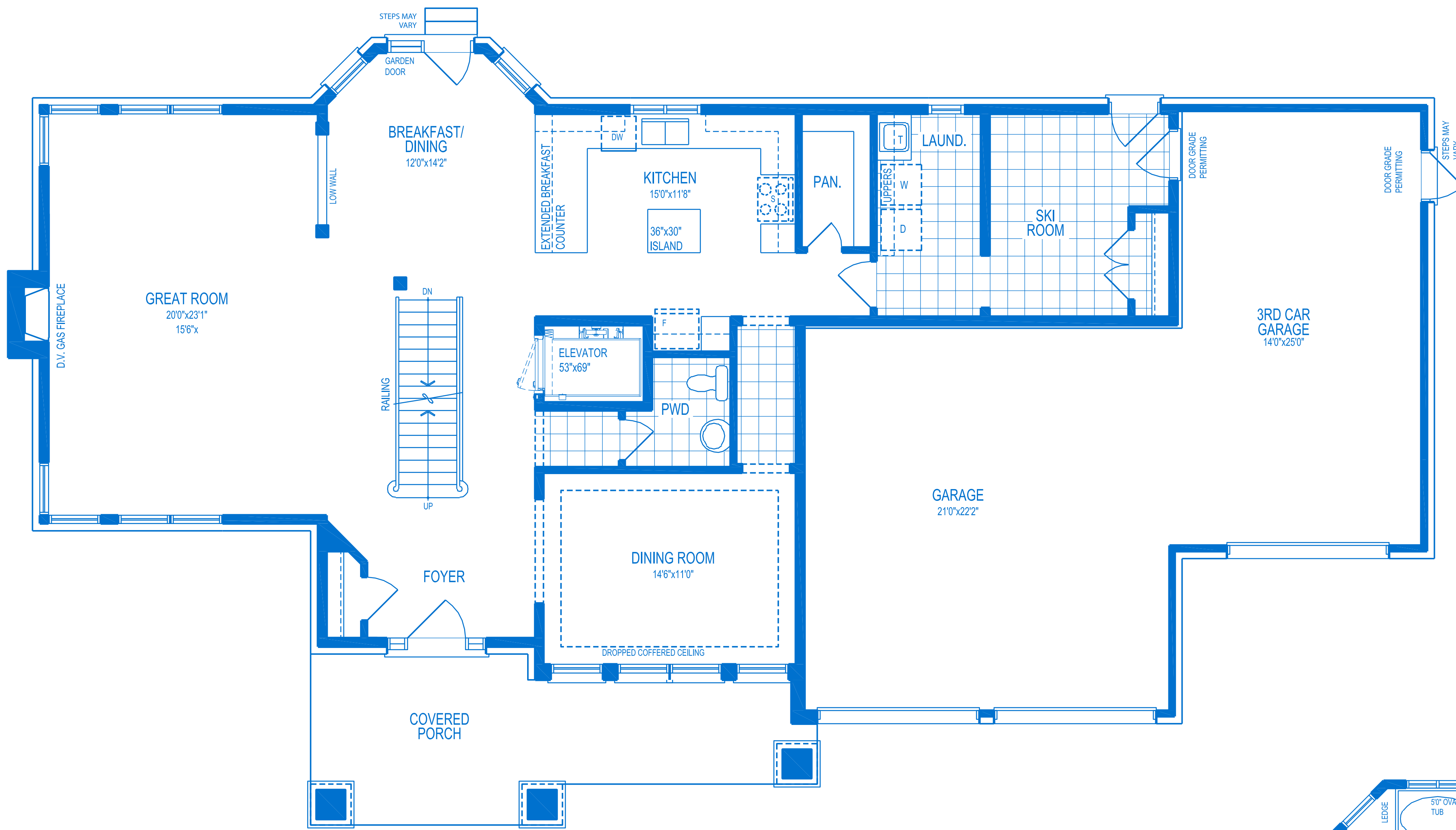
MAIN FLOOR PLAN, ELEV. 'C' W/ ELEVATOR
