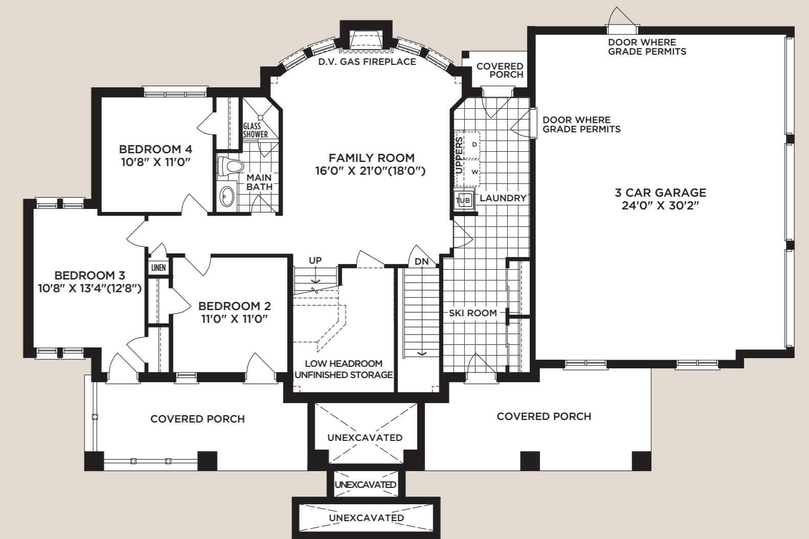
Main Level Elev A
